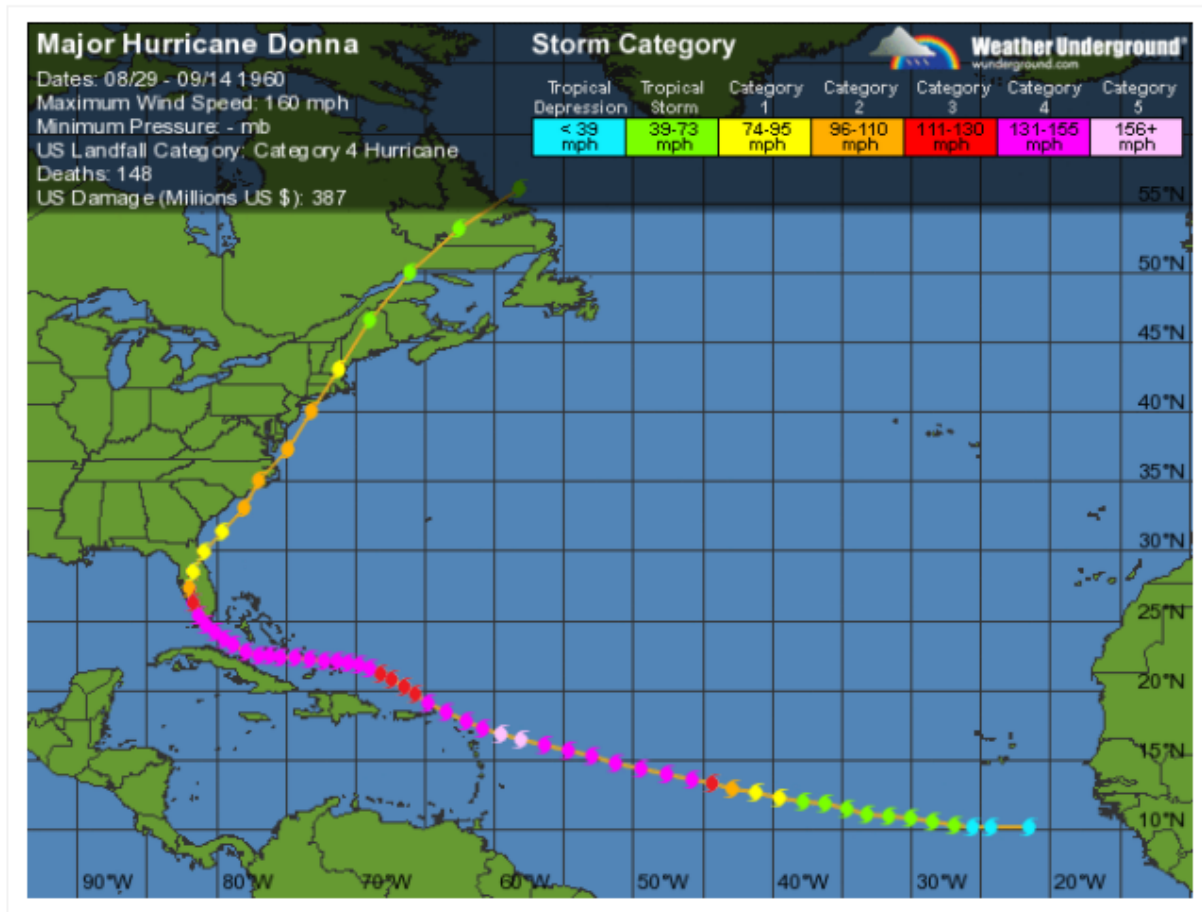
Figure 6. Track of Hurricane Donna of 1960.
